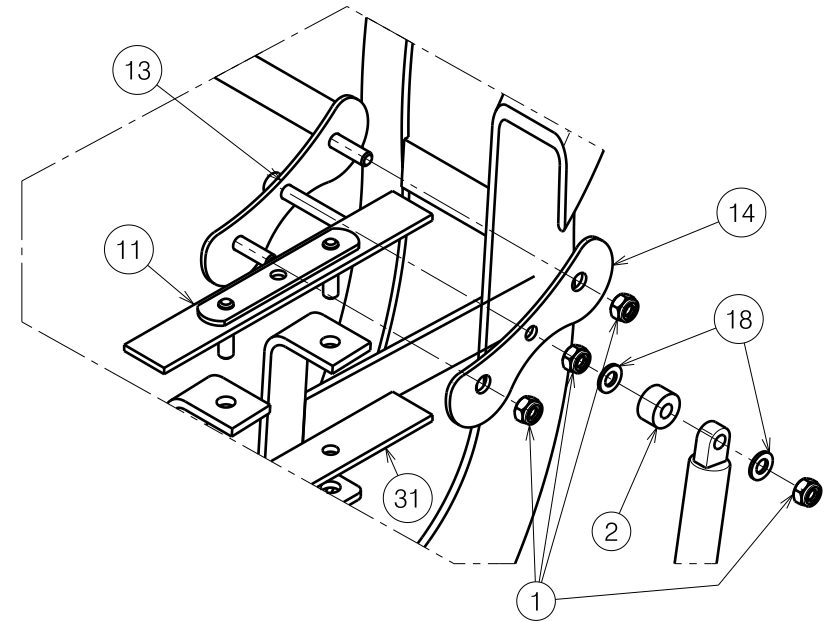
Detail A Scale / Schaal 1:4
